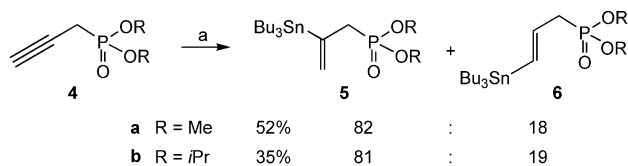
Scheme 2. Hydrostannation of propargylic phosphonates 4 . Reaction conditions: Bu 3 SnH (3 equiv.), hydroquinone (10 mol-%), MoBI 3 (2 mol-%), THF, 55 °C, (R = Me, 6 h; R = i Pr, 16 h).
