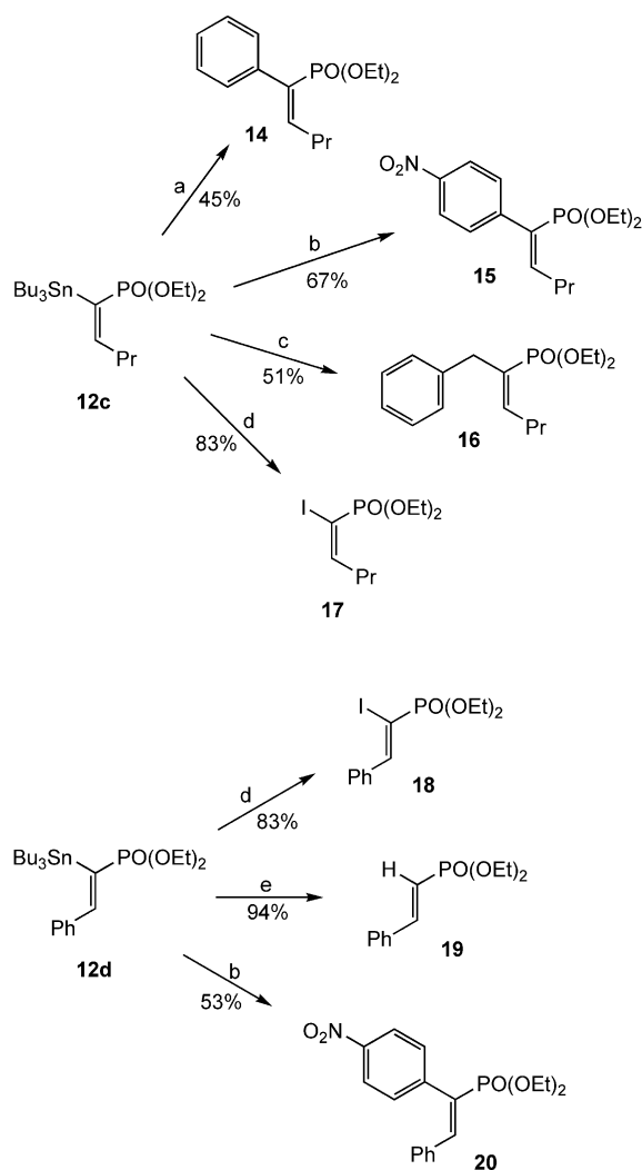
Scheme 4. Cross coupling reaction of stannated vinylphosphonates. Reaction conditions: a) PhI, CuI, Pd 2 (dba) 3 (2 mol-%), P(fur) 3 (15 mol-%), NMP, room temp., 16 h; b) p -NO 2 -PhI, CuI, Pd 2 (dba) 3 (2 mol-%), P(fur) 3 (15 mol-%), N -methylpyrrolidinone (NMP), room temp., 16 h; c) BnBr, Pd 2 (dba) 3 (2 mol-%), AsPh 3 (15 mol-%), toluene, 90 °C, 15 h; d) I 2 , CHCl 3 , room temp. 1 h; e) PhCOCl, [(allyl)PdCl] 2 /PPh 3 , THF, 60 °C.
