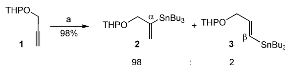
Scheme 1. Hydrostannation of alkyne 1 . Reaction conditions: a) \text{Bu}_3\text{SnH} (3 equiv.), hydroquinone (10 mol-%), \text{Mo}(\text{CO})_3(\text{CNtBu})_3 (2 mol-%), THF, 60 °C, 4 h.
