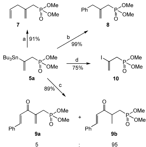
Scheme 3. Cross coupling reactions of stannated phosphonate 5a . Reaction conditions: a) Allyl bromide, [(allyl)PdCl] 2 /PPh 3 , THF, 60 °C, 16 h; b) Benzyl bromide, [(allyl)PdCl] 2 /PPh 3 , PPh 3 , THF, 60 °C, 16 h; c) cinnamoyl chloride, [(allyl)PdCl] 2 /PPh 3 , THF, 60 °C, 16 h; d) I 2 , CHCl 3 , room temperature, 1 h.
